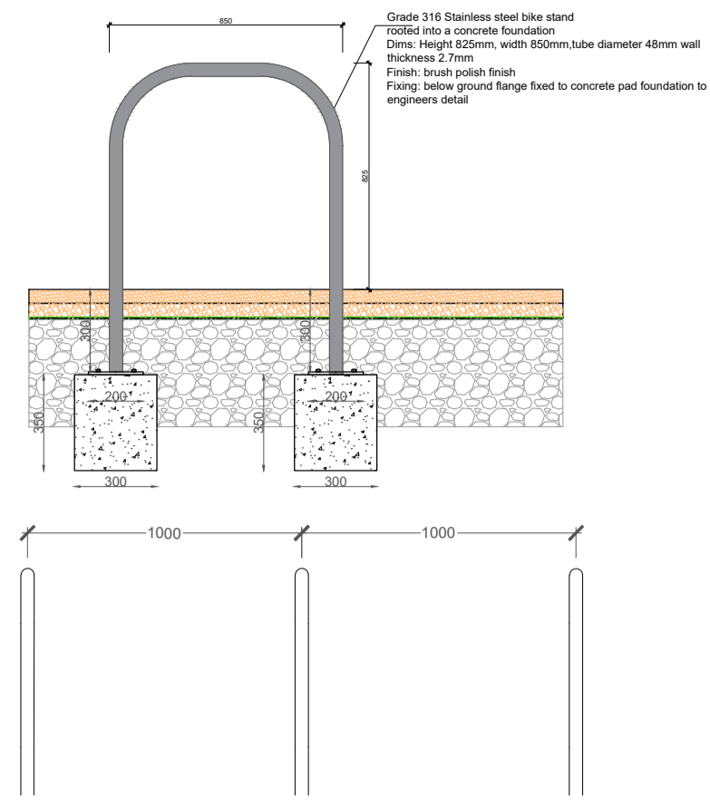
TYPICAL DETAIL - Sheffield cycling stand - 1/25 @A1
